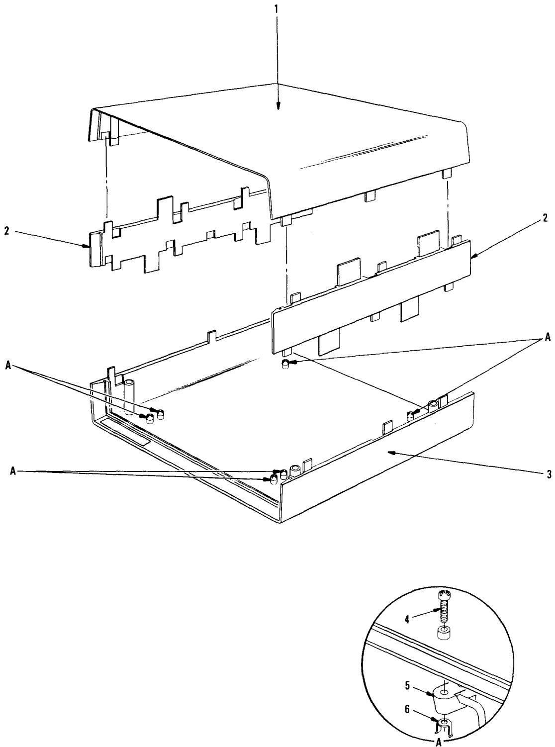
Figure 6. Cover Assembly.
