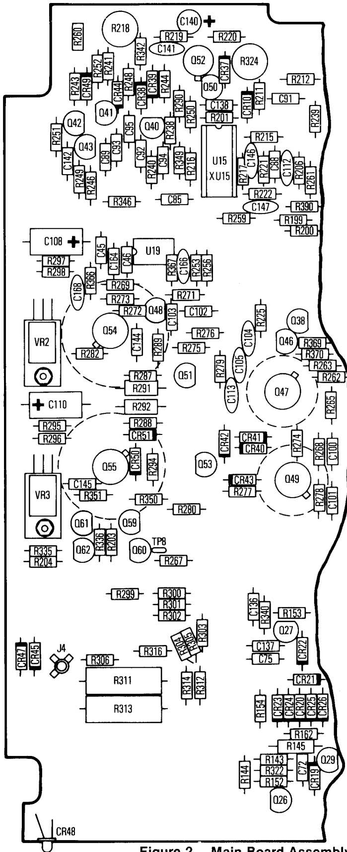
Figure 2. Main Board Assembly (Sheet 2 of 4).
