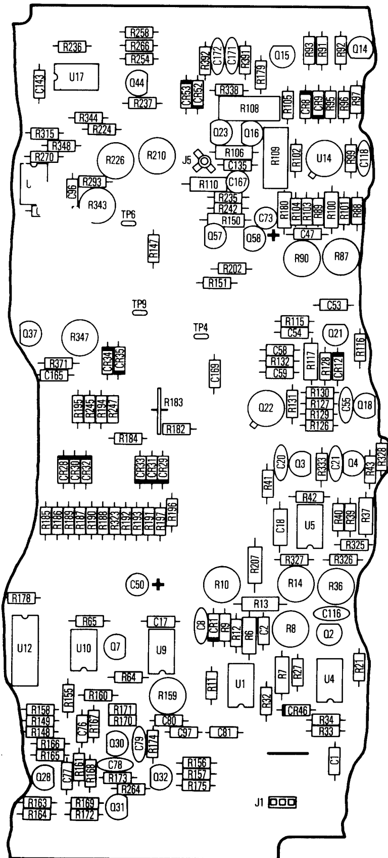
Figure 2. Main Board Assembly (Sheet 3 of 4).
